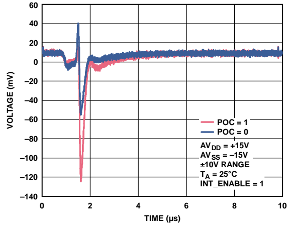
Figure 29. Voltage vs. Time on Output Enable
