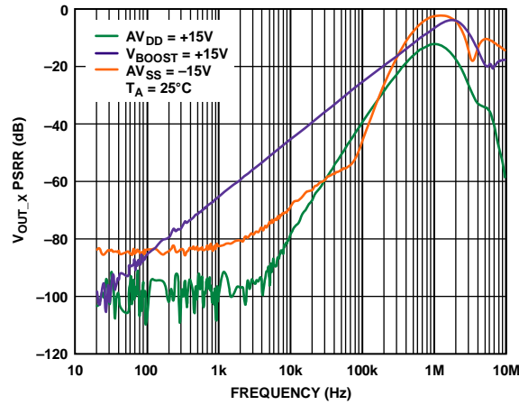
Figure 30. V_{OUT\_x} PSRR vs. Frequency
